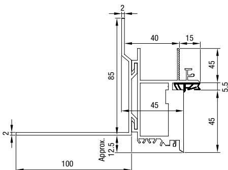
ZeroLine frame dimensions
