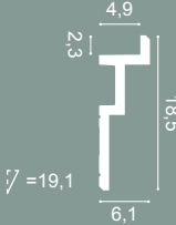
C396 STEPS 200 x 6,1 x 18,5 cm Purotouch ® Designed by Orio Tonini
