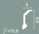
C321 | C321F 200 x 9,9 x 5 cm Purotouch ®
