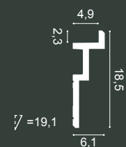
C396 STEPS 200 x 18,5 x 6,1 cm Purotouch ® Designed by Orio Tonini
