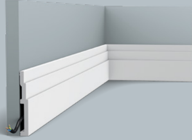
❷ SX180 | SX180F HIGH LINE 200 x 12 x 1,6 cm Duropolymer ® Designed by Pierre Daems
