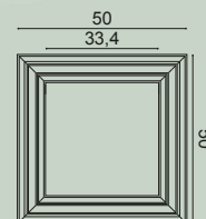
2 W121 AUTOIRE B 50 x 50 x 3,2 cm Purotouch ® Designed by Orio Tonini
