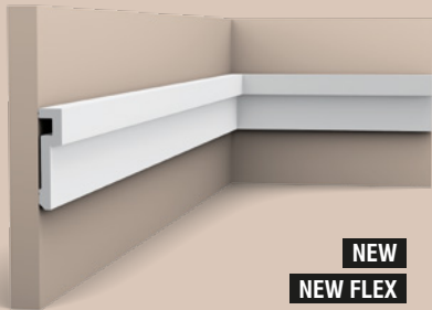
PX198 | PX198F U-STEPS 200 x 8,3 x 2 cm Duropolymer ® Designed by Orio Tonini
