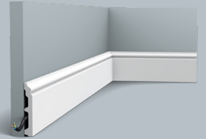
SX173 | SX173F | SX173-RAL9003 CONTOUR 200 x 10 x 1,6 cm Duropolymer ®
