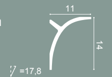
C991 200 x 14 x 11 cm Purotouch ® Designed by Ulrich Moritz
